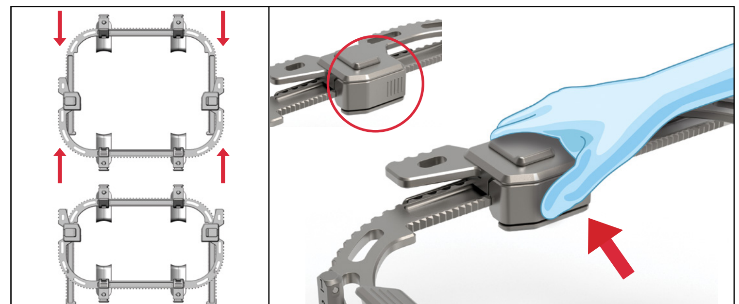
Push Inside Slide button to contract retractor
