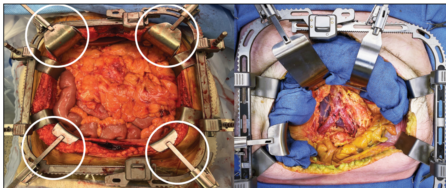
Bookwalter ® blades for enhanced stability and deeper exposure
